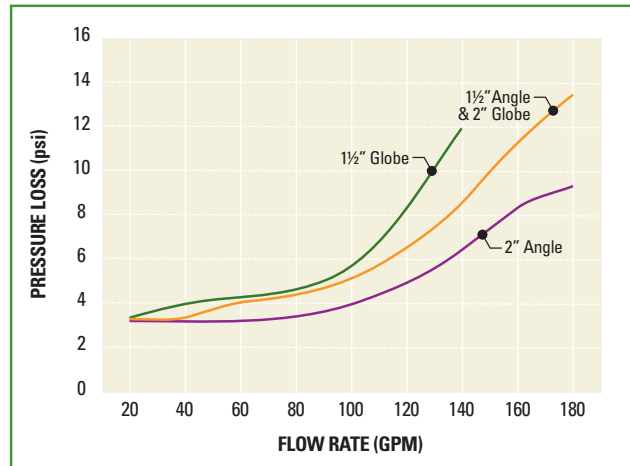
1 1/2" & 2" FLOW RATE VS. PRESSURE LOSS *
