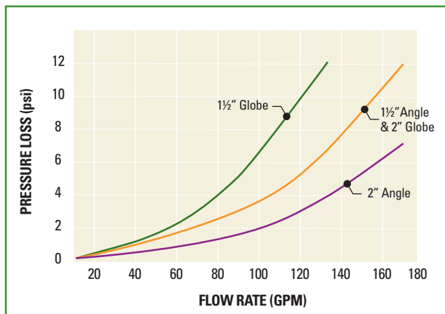
1 1/2" & 2" FLOW RATE VS. PRESSURE LOSS *
